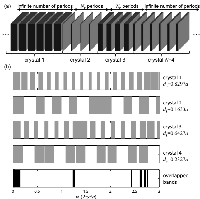
FIG. 1. (a) A photonic crystal heterostructure with four crystals. Each crystal has alternate silicon and vacuum layers, and a period a . The two crystals at either ends are assumed to be infinite. (b) In the top four panels, gray regions correspond to frequency ranges where the corresponding crystal, assumed to be infinite, has a propagating state along the normal incident direction. White regions are the band gaps. d_s is the thickness of the silicon layers. In the bottom panel, the black regions represent frequency ranges where there are photonic bands in all crystals.
